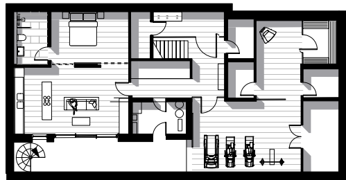
Basement
