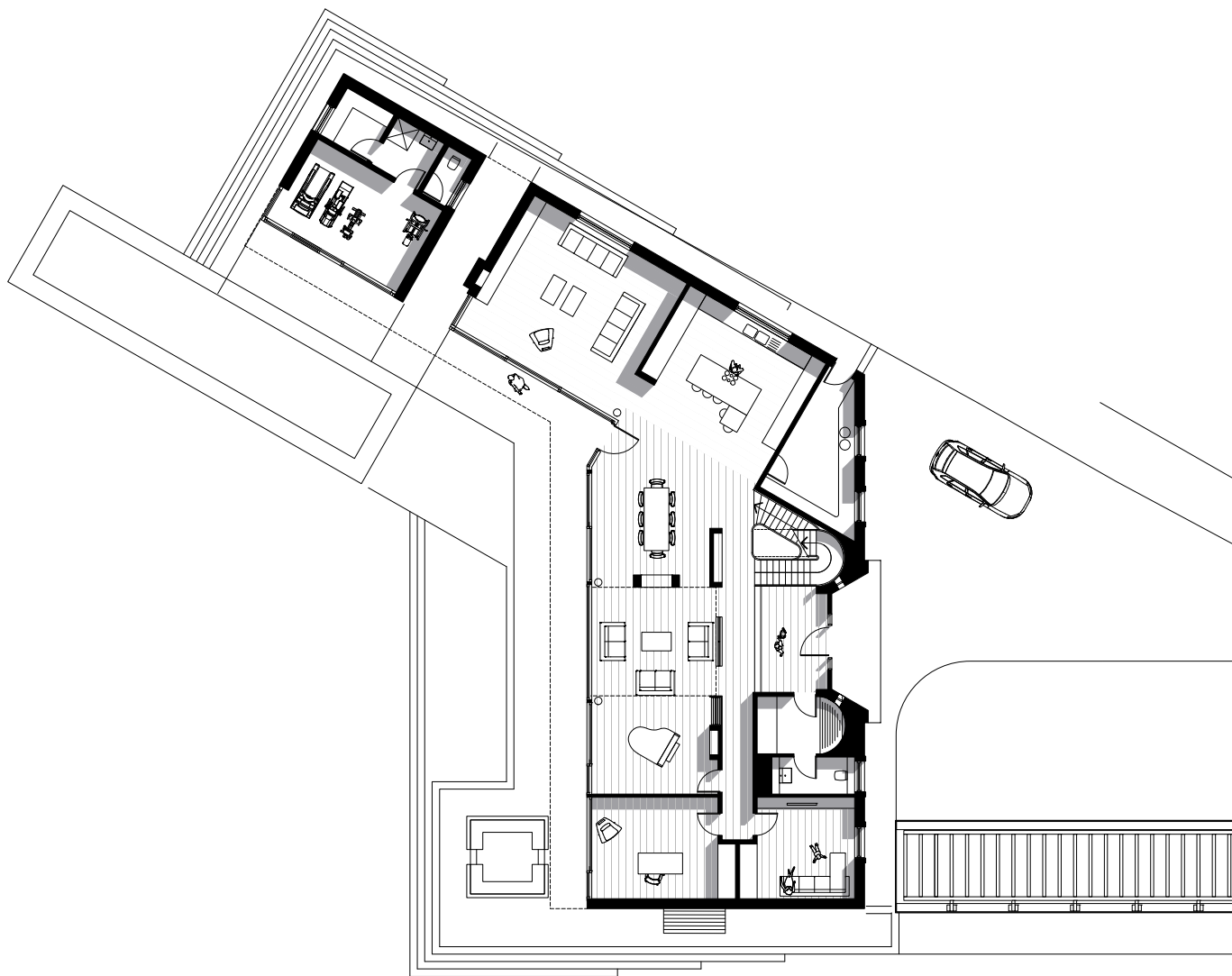
Ground Floor
