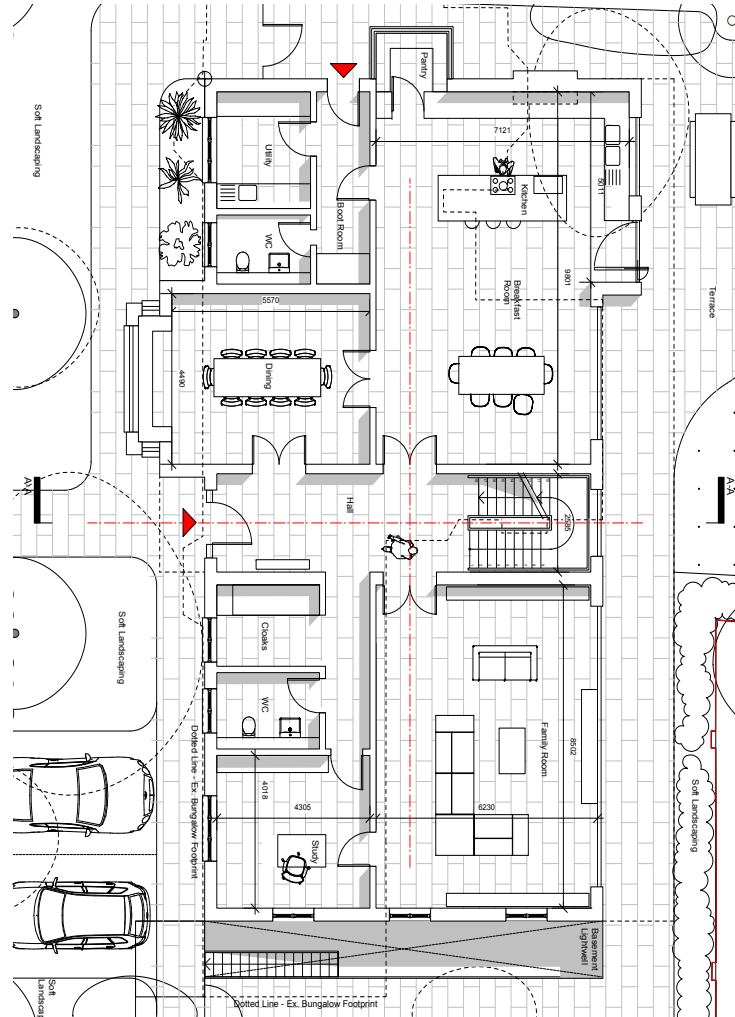
Ground
